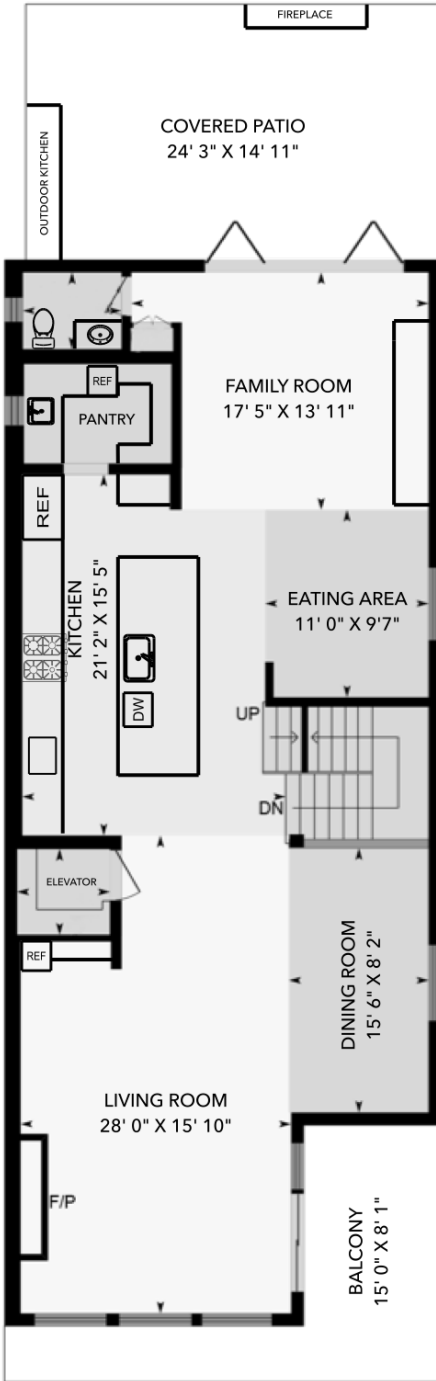
MAIN LEVEL 1486 SQ.FT. CH: 17' 6"/8' 11"
